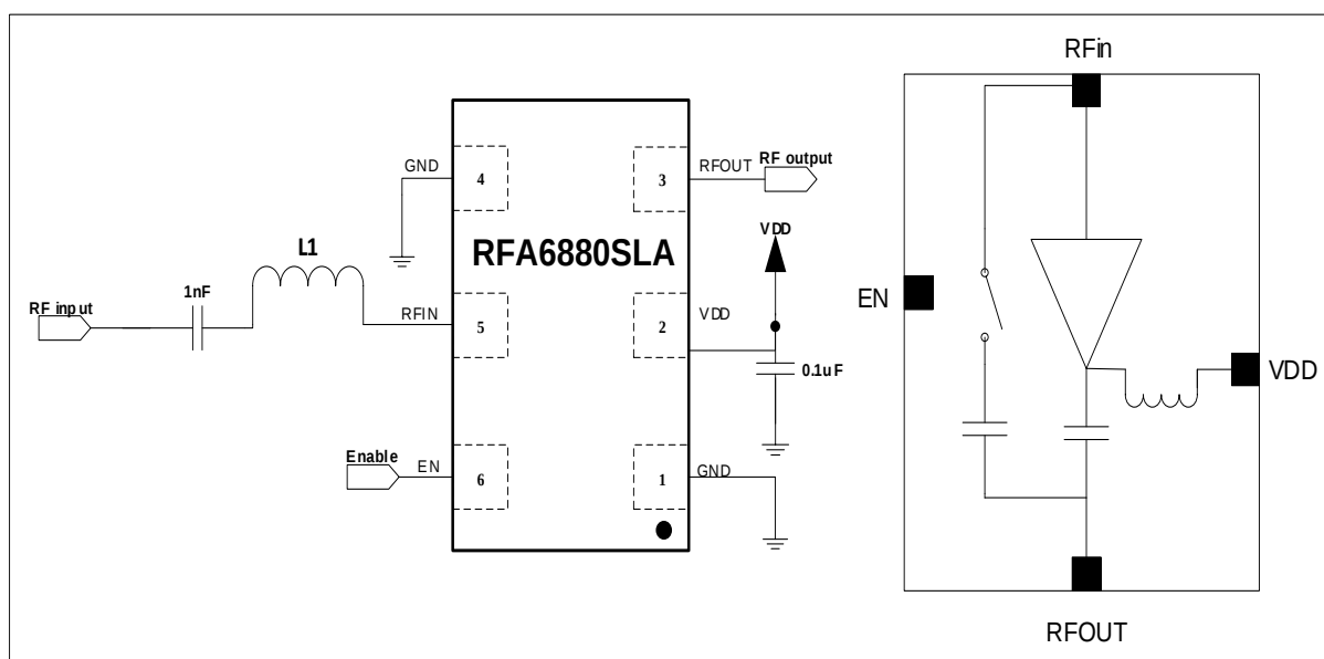
Figure 1 RFA6880SLA application circuit
